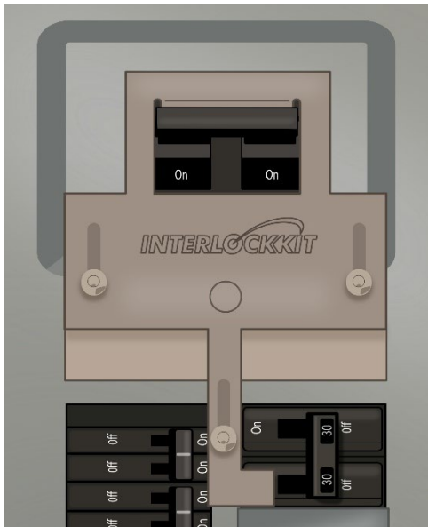
Main Breaker ON
