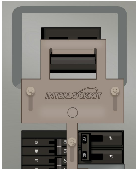
Generator Breaker ON
