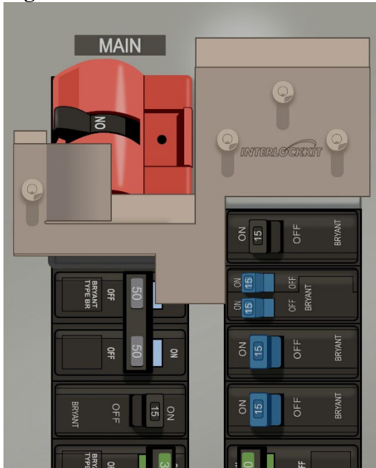
Main Breaker ON
